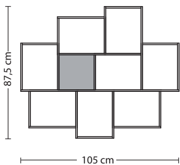
Coffee table 105 - with 1 inlay - top view
